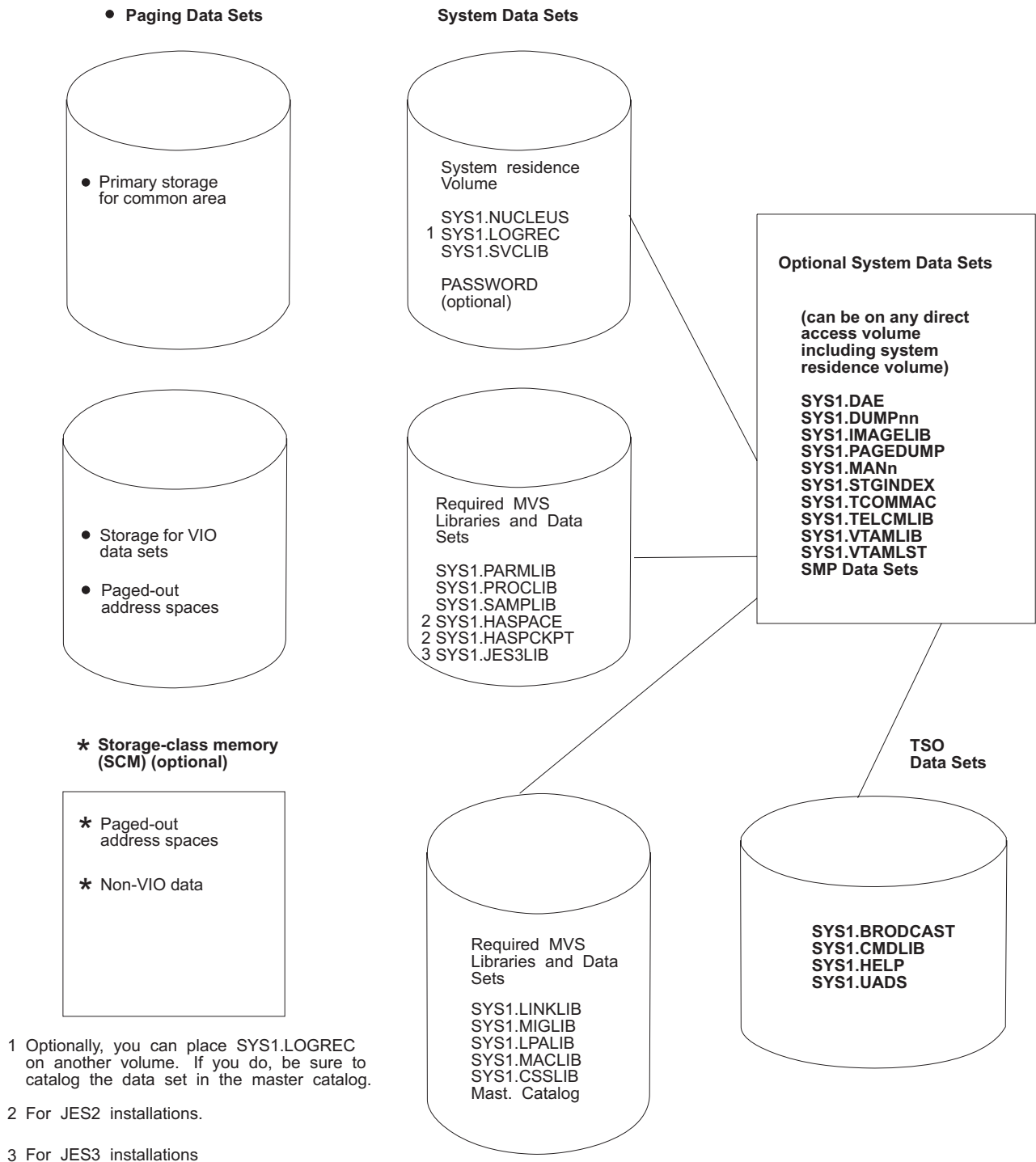
Figure 4. Auxiliary storage diagram with SCM
